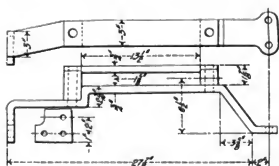
Figs. 2730-2731. Trailing Truck Cylinder Beam Guide.
